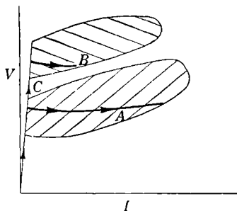
Fig. 8.13.—Mode skip determined by speed of starting in the lower mode.
